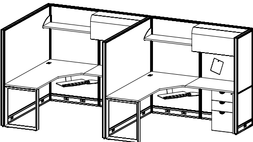
COMPLETE LAYOUT COMBINES FRAMEWORK W/ HDL INNOVATIONS SERIES (REFER TAB INV)
