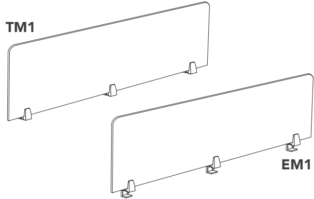
(3 brackets per panel & 2" insets from each end)
